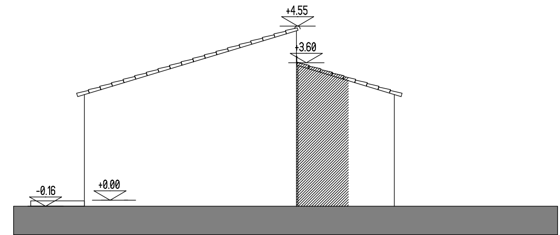
FACADE SUD
